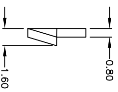
LOCK WASHER (2 PCS)
